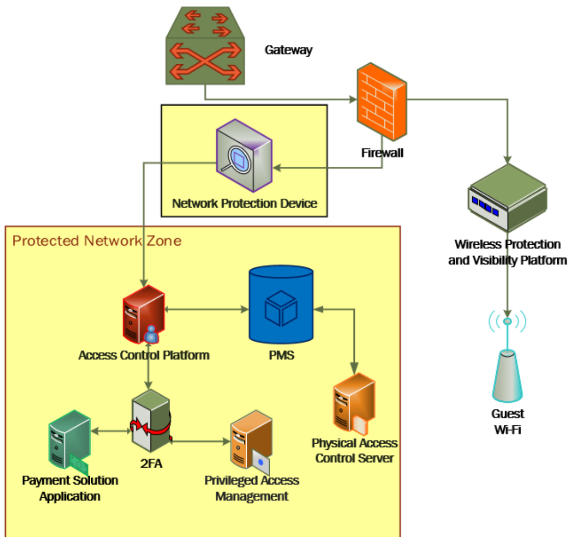
Figure 2-1 Network Protection Solution in the Reference Architecture
