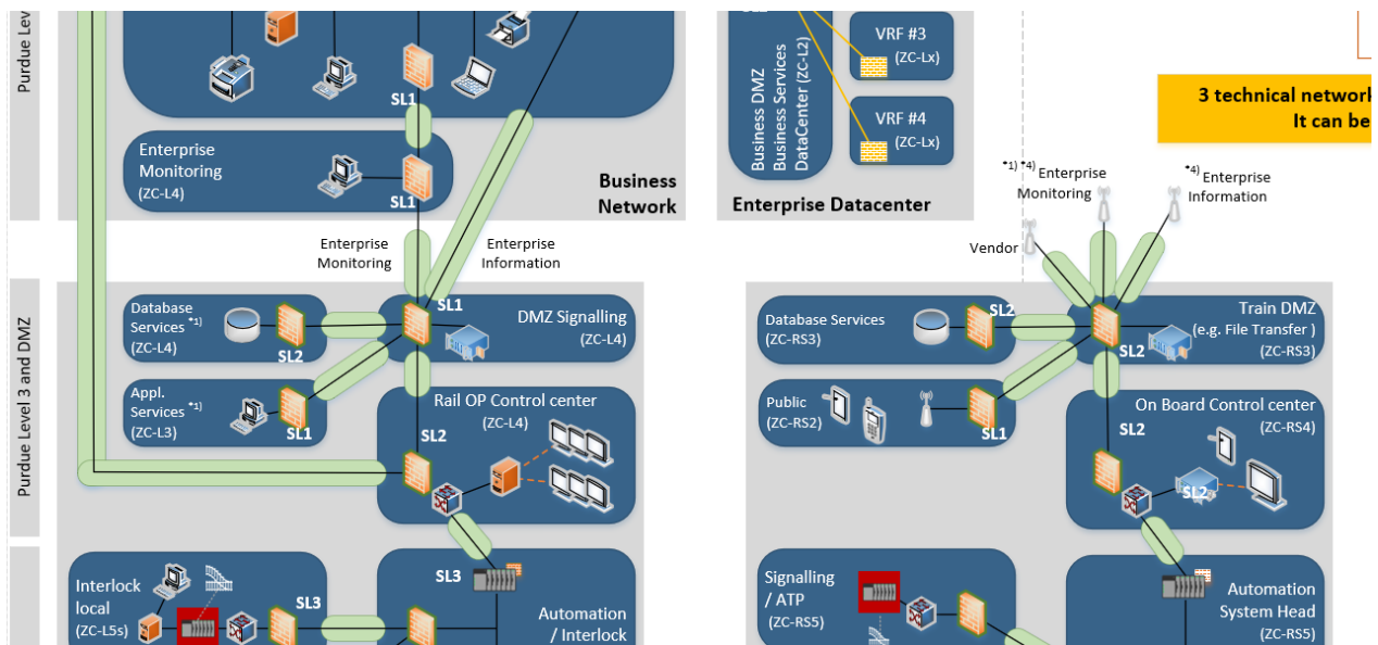
Figure 15 Example of defining SL to each zone and conduit
