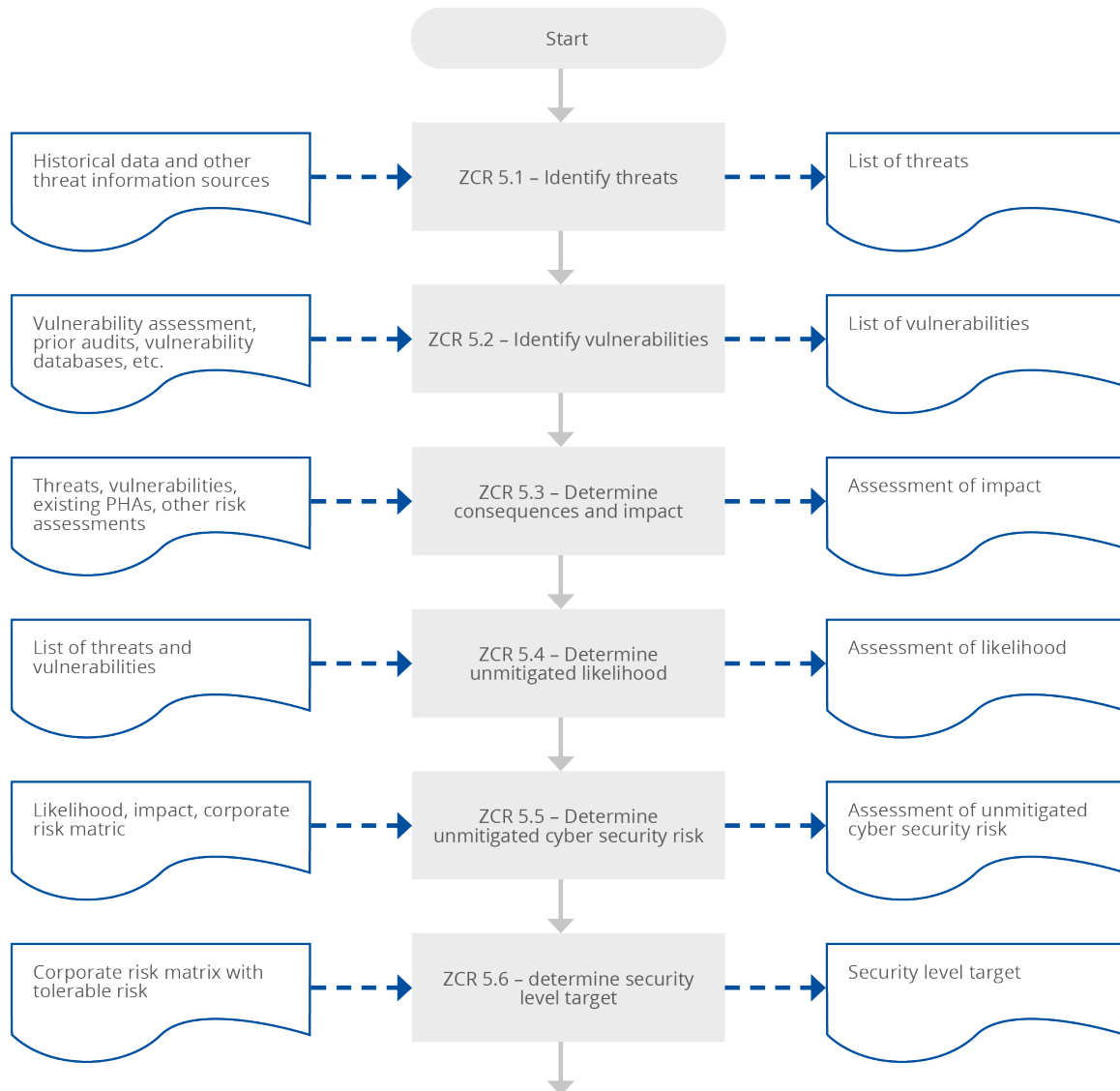
Figure 18 Detailed risk assessment steps
