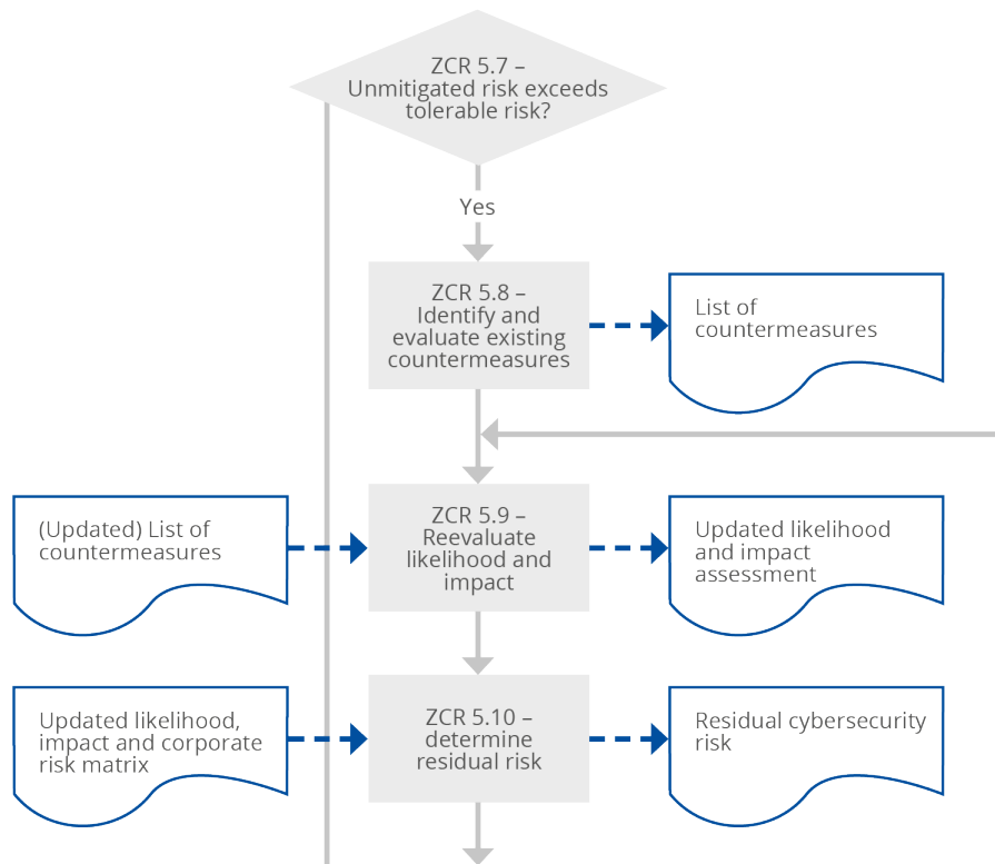
Figure 19 Process of identifying countermeasures
