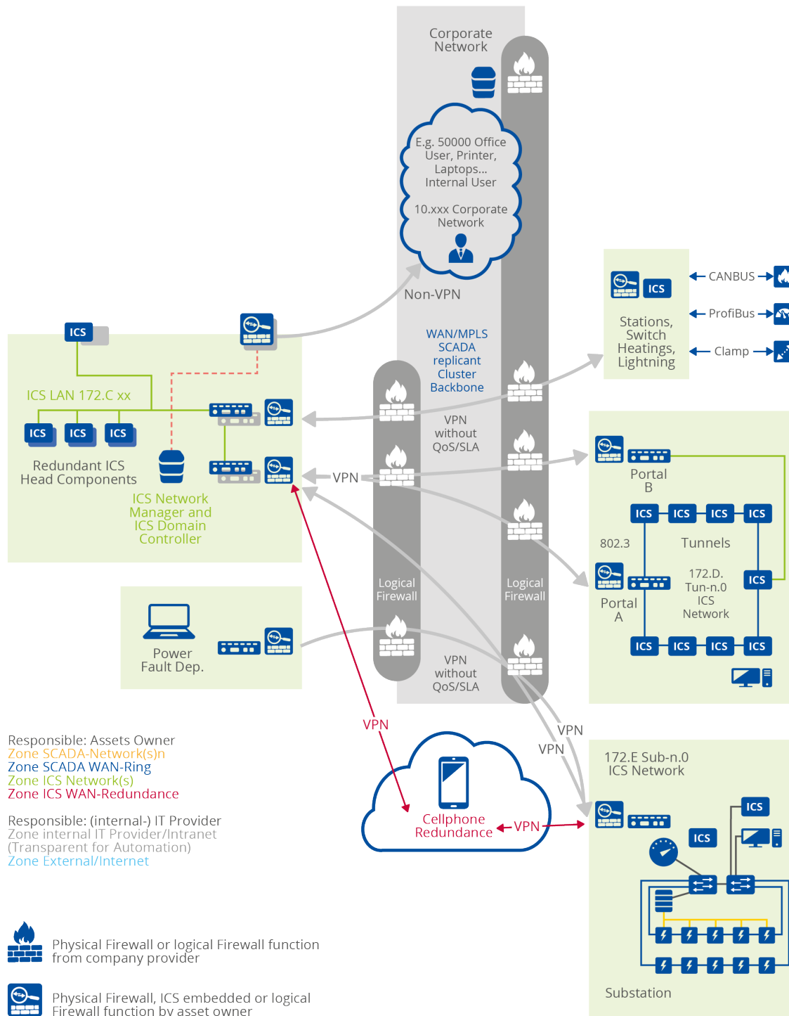
Figure 14 Example of transparent communication lines between zones
