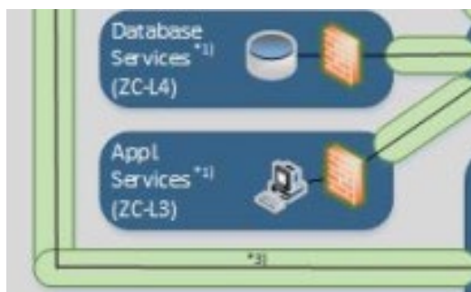
Figure 11 Example of defining zone criticality in the individual railway zone model
