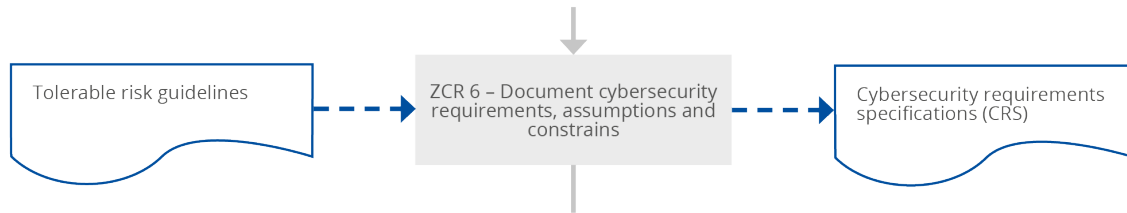
Figure 21 Documenting cybersecurity requirements (ZCR 6)
