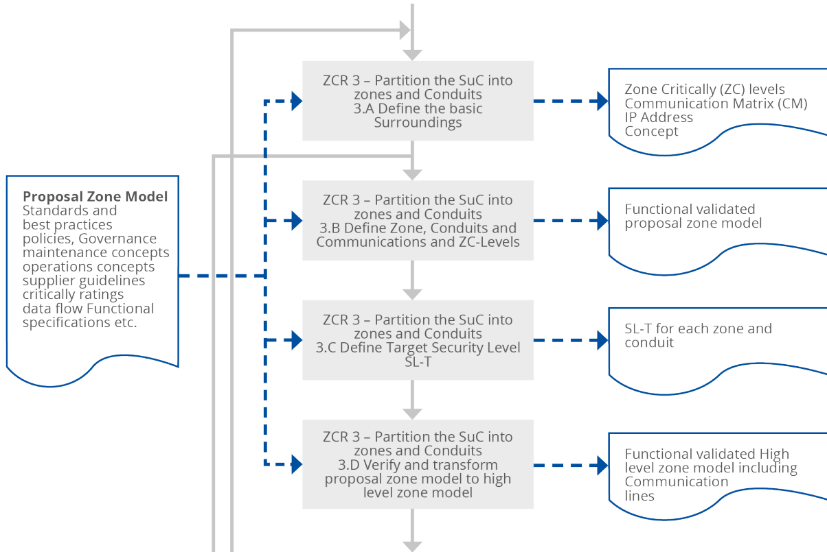
Figure 9 Partitioning and SuC process (ZCR 3)
