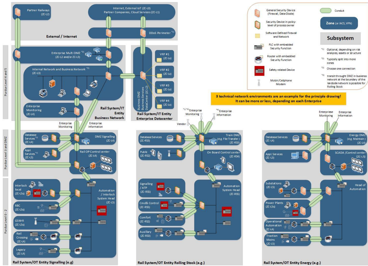
Figure 10 Example of an individual railway zone model
