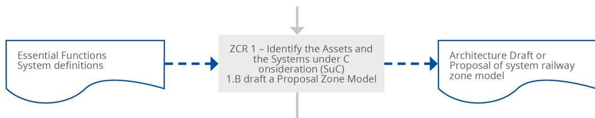
Figure 5 Proposal zone model with all assets and communication information
